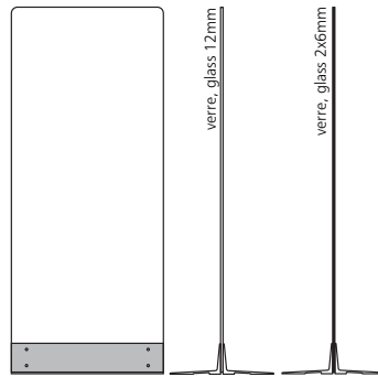
île 223 S w 750 x h 1800 x d 512mm w 29,52 x h 70,86 x d 20,15° île 123 S w 750 x h 1800 x d 512mm w 29,52 x h 70,86 x d 20,15°
