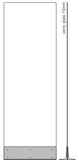
île 336 S w 1000 x h 3000 x d 315mm w 39,37 x h 118,11 x d 12,40°
