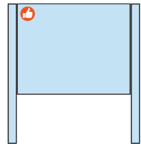
Post and panel Sign Panel: 1 Post: 2/Ø= 90 mm / 3.5" Windload A1, A2, B1, B2
