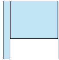
Post and panel Sign Panel: 1 Post: 1/Ø= 90 mm / 3.5" & 1/ID 175 mm / 6.875" Windload A1, A2, B1, B2
