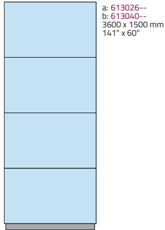
Monolith 104 mm / 4.1" Windload: A1, B1
