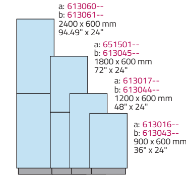
Monolith 53 mm / 2.1" Windload: A1, A2, B1, B2
